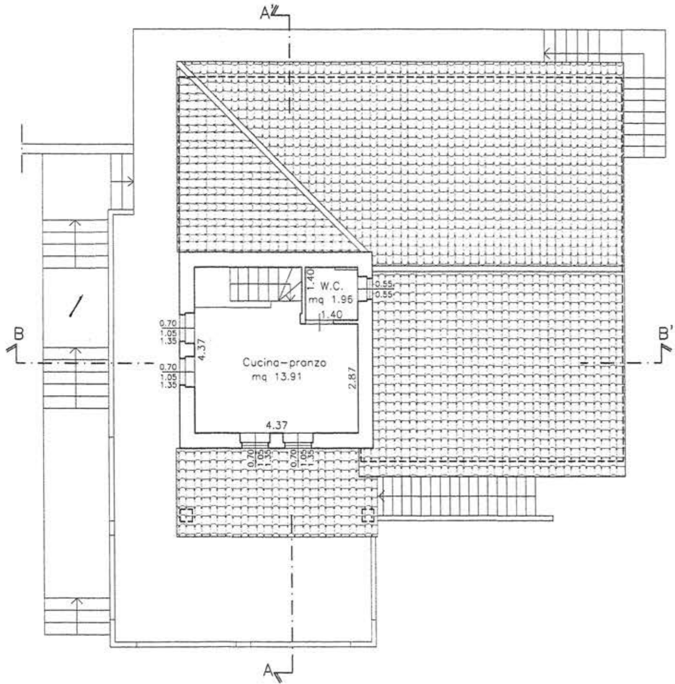
PIANO COLOMBAIA
